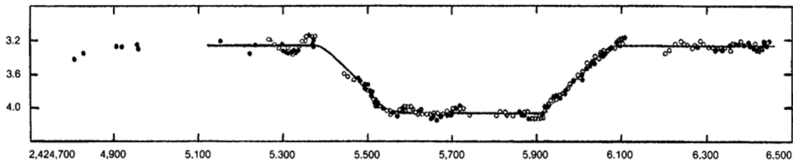
Figure 1b. 1928-30 ECLIPSE - JD 2,424,700 to JD 2,426,500) Ref: Reddy, Sky & Telescope May 1982 p. 460. (Data from Güssow, Stebbins, and Huffer).
